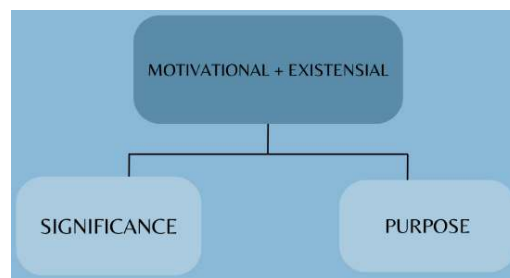
Figure 5.2.1: Motivational plus Existential parse into Significance or Purpose
