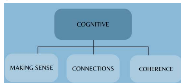
Figure 5.2.1: Cognitive Flow parse into 3 areas; Motivation, Connections or Coherence
